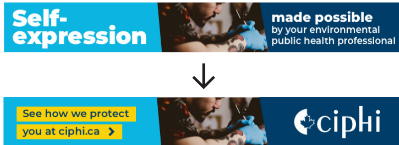
Leaderboard (animated)
